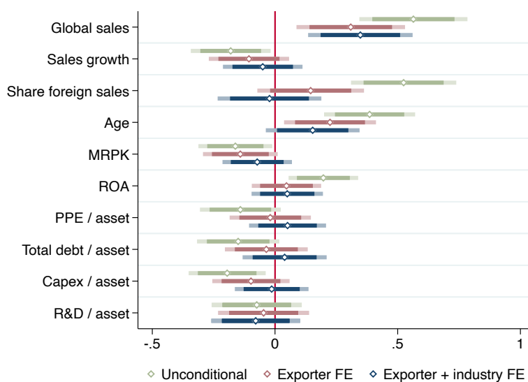
Figure 2: Covariate Balance
