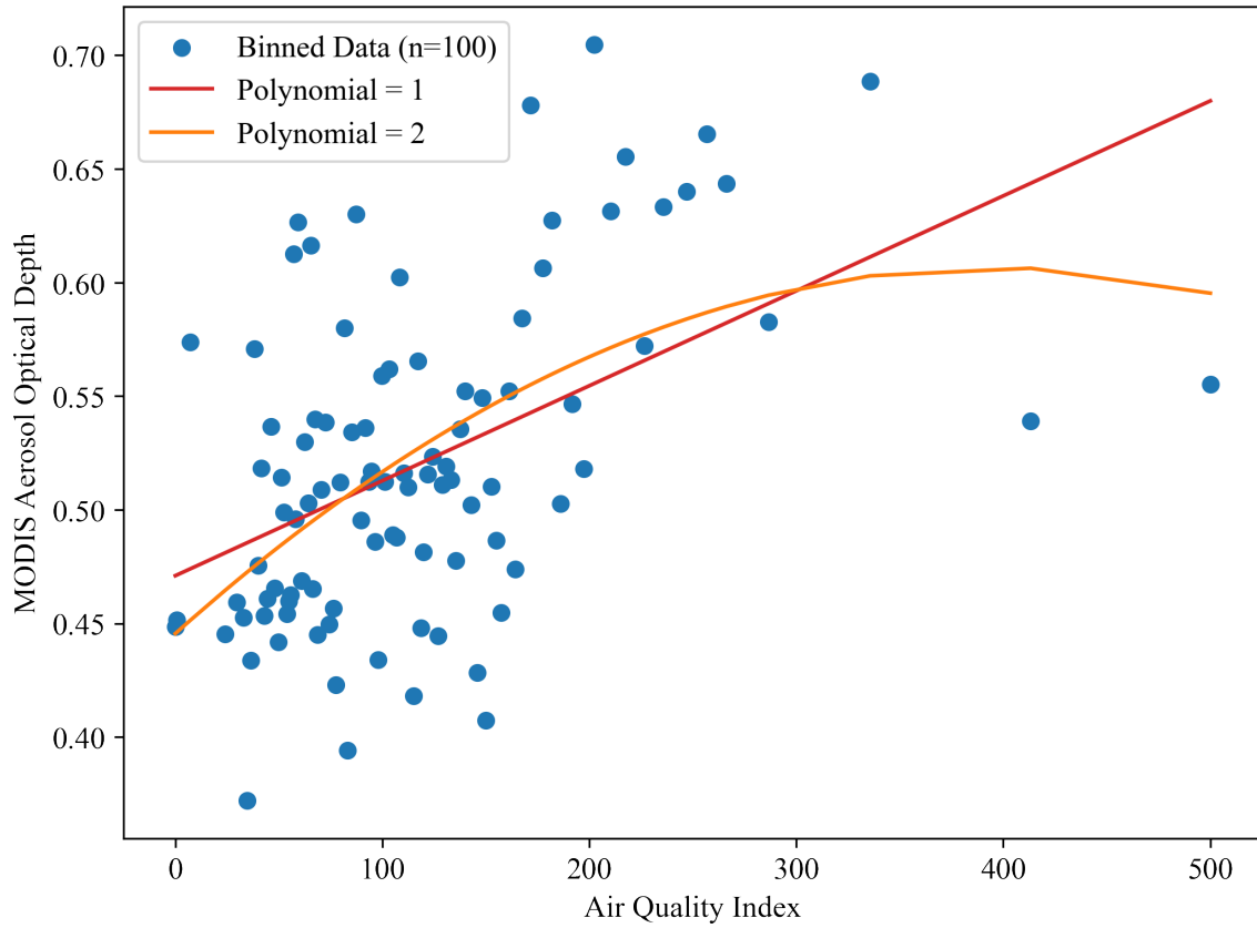
Figure A5: Correlation between AOD and AQI: Binned Scatterplot
