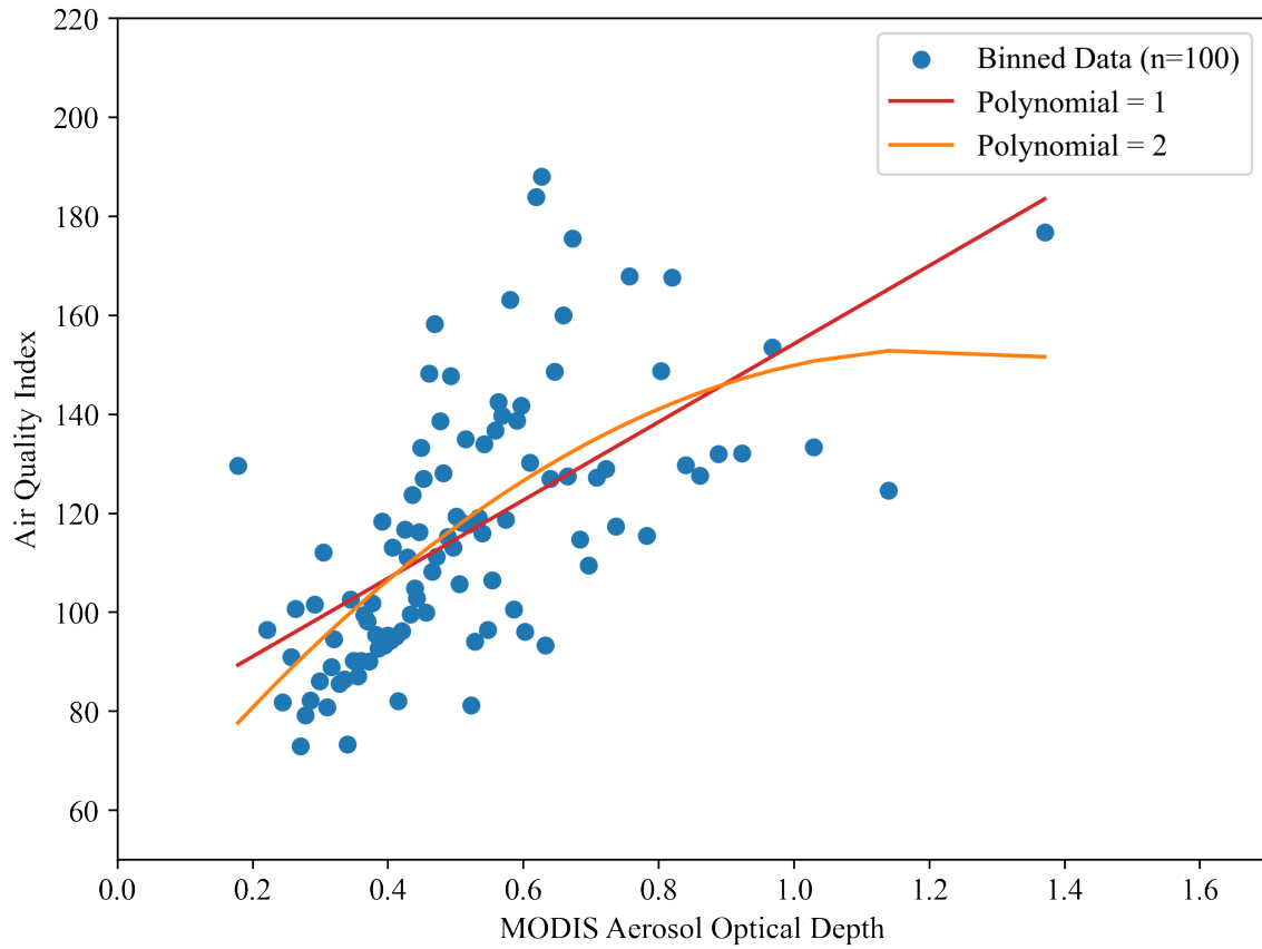
Figure A3: Correlation between AQI and AOD: Binned Scatterplot
