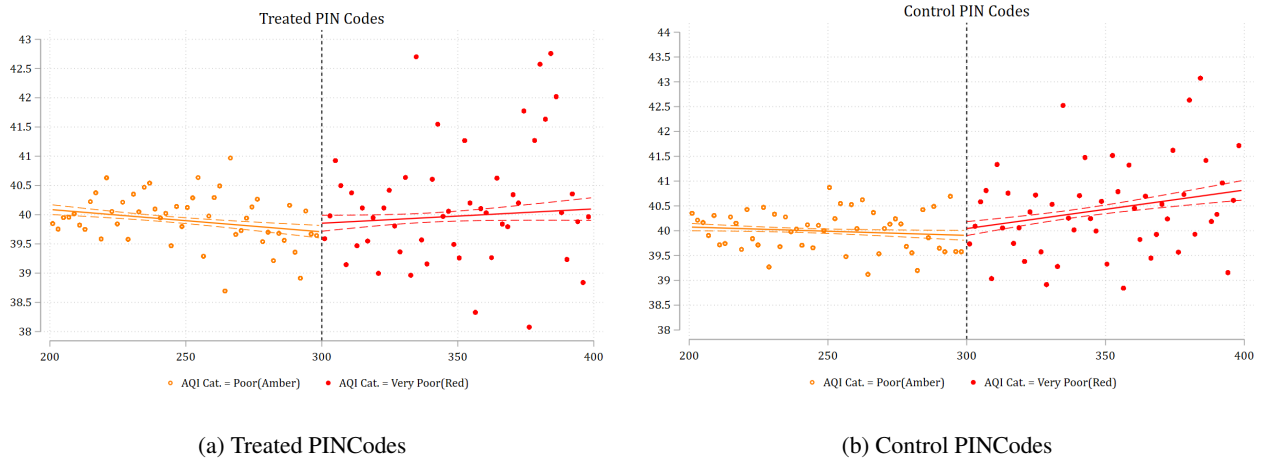
Figure A6: RD Plots for Brown Share versus AQI: Transition from Amber to Red
